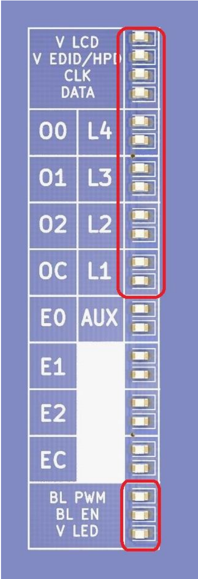
LVDS 1ch (HD) 40 pin LED
